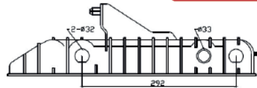
DPI-1786 2 3/8 X 18 5/8 AUT/T. ASTRO/SAFARI VAN 95-02
