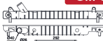
DPI 2458 2 1/4 X 27 1/2 TRAIL BLAZER/BRAVADA 02/07
